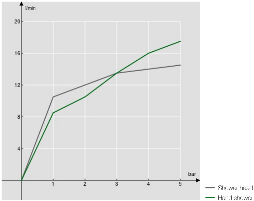
FLOW RATE DIAGRAM: HOT/COLD WATER
